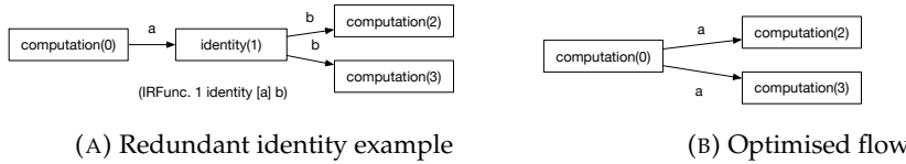
FIGURE 8.2: Optimising identity operators
