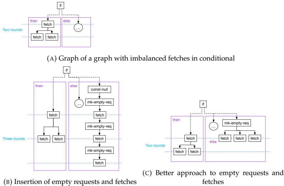
FIGURE 6.4: Two approaches to inserting empty fetches
