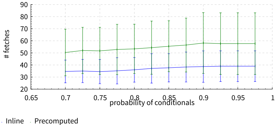
FIGURE 11.6: Number of fetches performed
