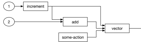
FIGURE 3.2: An example for code transformation in Ohua
