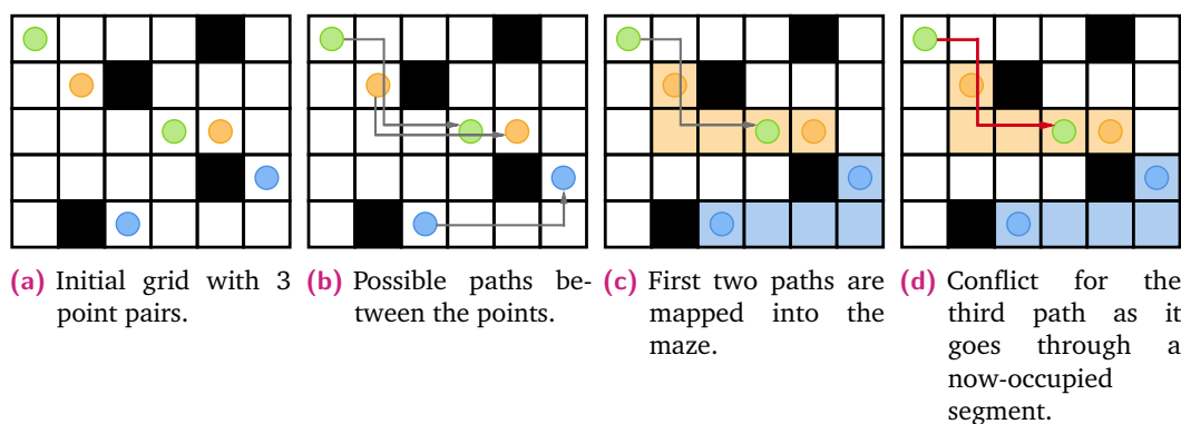
Fig. 3.1: Illustration of the operation of the labyrinth benchmark, showing the (attempted) mapping of 3 paths in a 6 \times 5 two-dimensional grid. Black squares represent walls that cannot be routed through.
